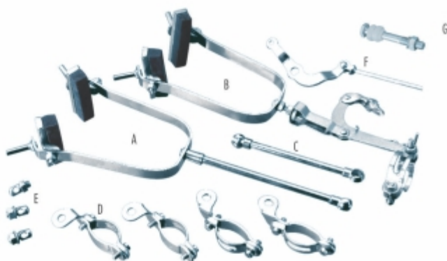
VI-393 BRAKE SET PH. TYPE (A) Front Stirrup with Tube & Brake Shoe. (B) Rear Stirrup with Adjustable Bolt & Bottom Leg Unit with Clip & Spring. (C) Rear Brake Tube with Screw. (D) Brake Clip Front with Screw & Nut (E) Brake Button with Nut & Washer (F) Rear Brake Long Connecting Rod with Bell Crank Lever (G) Frame Bolt
