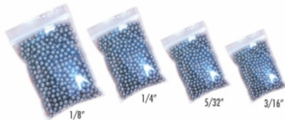
STEEL BALLS 5/32" : For Fork Fitting 3/16" : For Front Hub 1/4" : For Rear Hub 1/4" : For B.B. Fitting
