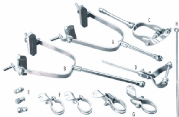
VI-394 BRAKE SET RL. TYPE (A) Front Stirrup with Tube & Brake Shoe. (B) Rear Stirrup with Tube & Brake Shoe. (C) Top Ball Crank with Pin & Tube. (D) Bell Crank & End Pin. (E) Brake Button with Nut & Washer (F) Brake Clip Rear with Screw & Nuts. (G) Brake Clip Front with Screw & Nuts. (H) Rear Brake Long Connecting Rod with Round Ends.
